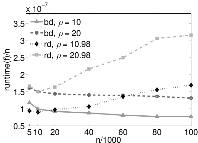
Figure 8: Runtime of function evaluation in seconds normalized by input size n versus n .
