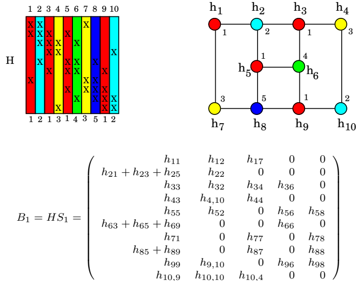
Figure 1: Top—a symmetrically orthogonal partition of the columns of a Hessian and its representation as a star coloring of the adjacency graph. The illustration uses five colors—red, blue, yellow, green and navy blue—which are also represented by the integers 1, 2, 3, 4 and 5, respectively, as shown at the bottom edge of the matrix as well as adjacent to the vertices of the graph. Bottom—the compressed matrix obtained by adding together columns that belong to the same group in the partitioning.
