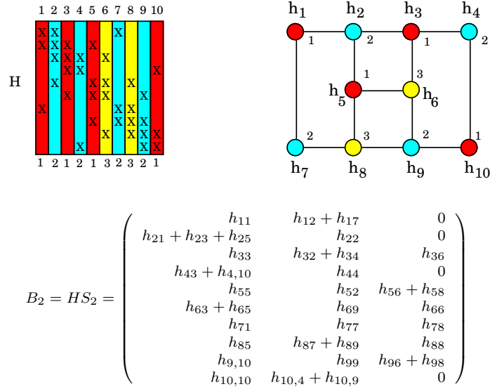
Figure 4: Top—a substitutable partition of the columns of a Hessian and its representation as an acyclic coloring of the adjacency graph. The illustration uses three colors—red, blue and yellow—which are also represented by the integers 1, 2 and 3, respectively, as shown at the bottom edge of the matrix as well as adjacent to the vertices of the graph. Bottom—the compressed matrix obtained by adding together columns that belong to the same group in the partitioning.
